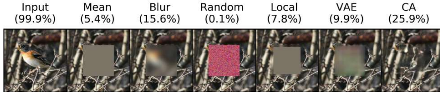
Figure 14: Different filling techniques for image parts, along with the resulting model activation of the class of interest. Generative models (VAE, CA), reconstruct the images with a more friendly and natural fill.
