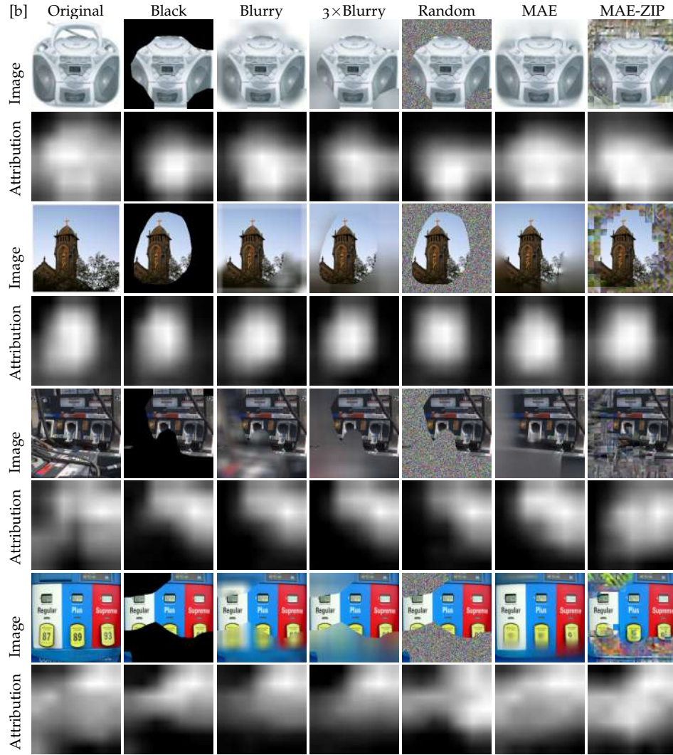
Figure 29: A visual comparison of the examined filling techniques.
