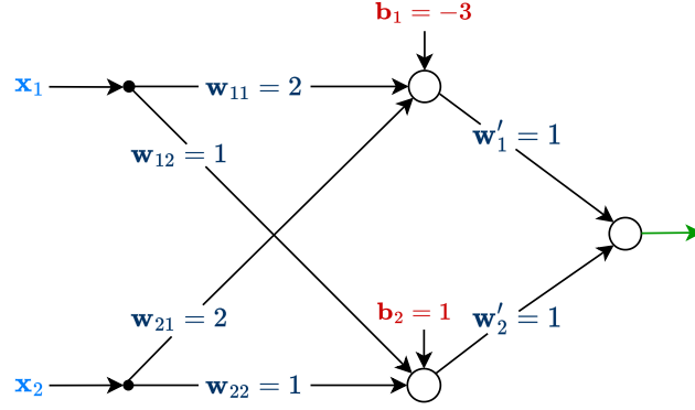
Figure 23: In the architecture presented, if x_1 = 1, x_2 = 0 , the upper neuron in the hidden layer becomes deactivated, preventing input x_1 from contributing through the upper path. To satisfy both fundamental criteria, the values of x_2 need to be determined in a way that ensures their dual purpose.
