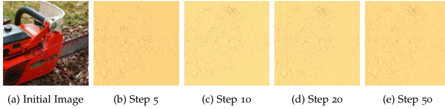
Figure 19: The evolution of the attribution map for the initial image (a), as the number of steps increases. The behavior of the attribution remains predictable, yet the random noise increases as the number of steps grows.
