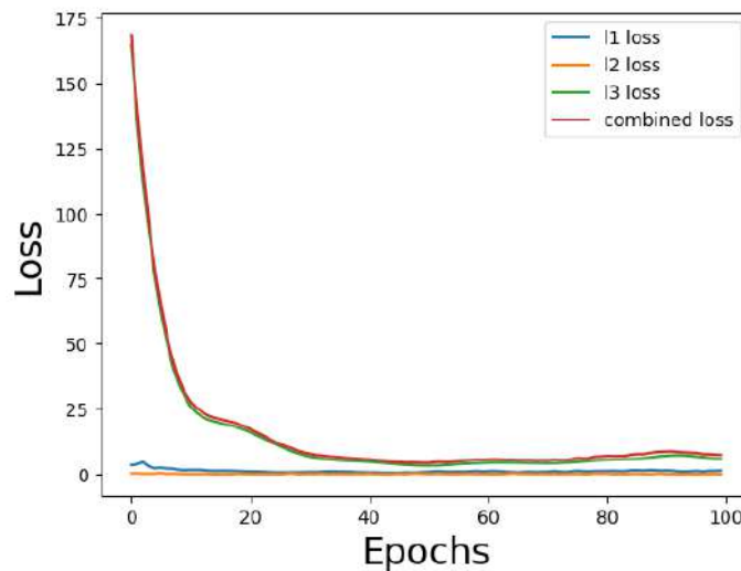
Figure 27: The plot of the losses when all combined together, for the standard set of hyperparameters.
