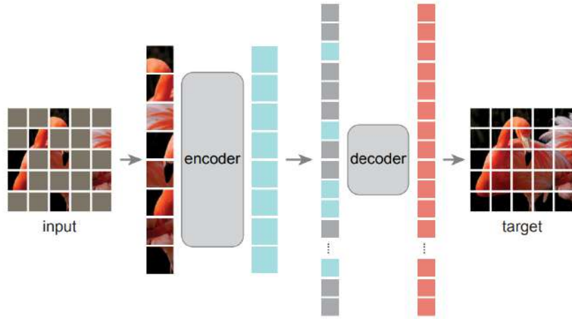
Figure 15: The architecture of MAE autoencoders and the asymmetric encoder-decoder sequence.
