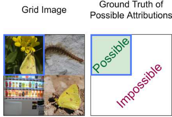
Figure 7: The 2 \times 2 grid for a particular set of images. As the annotator image on the right shows, only the image that contains the object(s) of a particular class can have a possible attribution.
