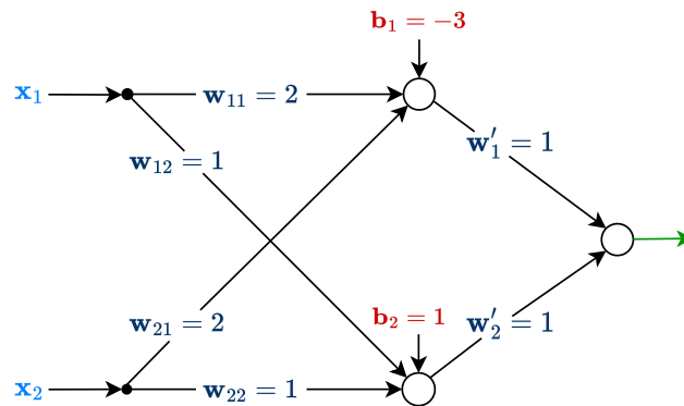
Figure 12: The Attribution shift problem is noticeable in this neural network architecture with one hidden layer and ReLU activation functions. If x_1 = x_2 = 1 , both neurons of the hidden layer are activated, and the two inputs contribute to the output from both the upper and lower path. But, if x_1 = 1, x_2 = 0 , the upper neuron of the hidden layer is deactivated, thus input x_1 cannot contribute from the upper path. It now contributes less to the model decision, leading to a drop in its attribution score.
