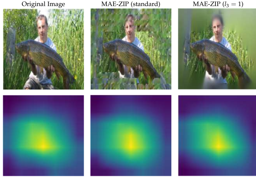
Figure 28: displays the original image along with the reconstructed images for two different setups in the first row, namely the standard and one with a highly biased to the third loss, along with their corresponding GradCAM attributions in the second row.
