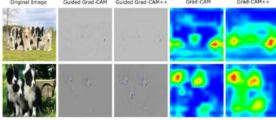
Figure 3: GradCAM and GradCAM++ in action.
